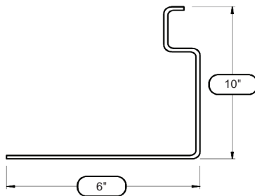
LANDING RISER
