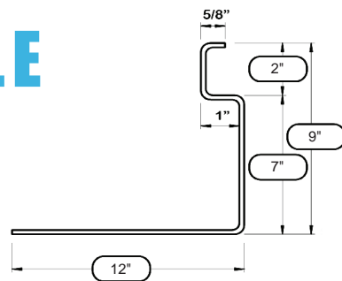
COMBINATION TREAD & RISER
