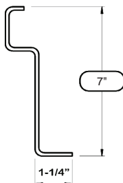
STARTER RISER
