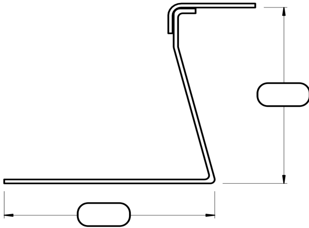
Nominal Tread (not including 1" nosing)
