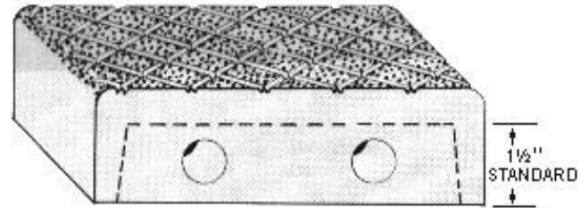
TYPE 117A Double Nose – 1 1/2" standard DRAWING NOT TO SCALE
