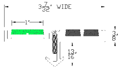
TYPE 630B-NG 3 7/32" wide, 3/8" thick DRAWING NOT TO SCALE
