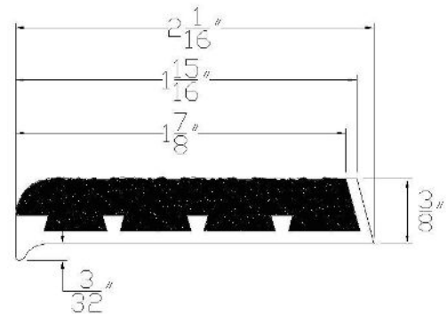
Type WP2JT
