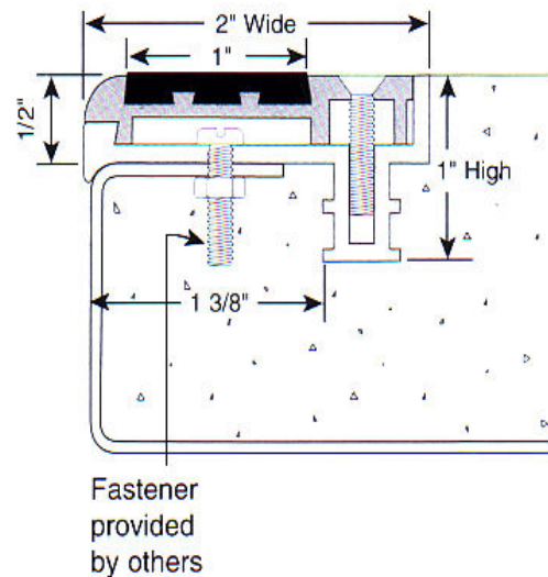
Type WP-RN2-SP 2" wide, 1/2" thick, sure-hold anchor DRAWING NOT TO SCALE
